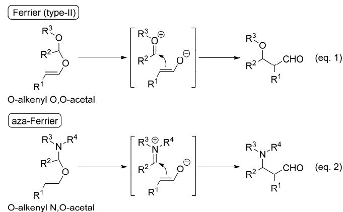
Scheme 1 Ferrier (type-II) and aza-Ferrier reaction
