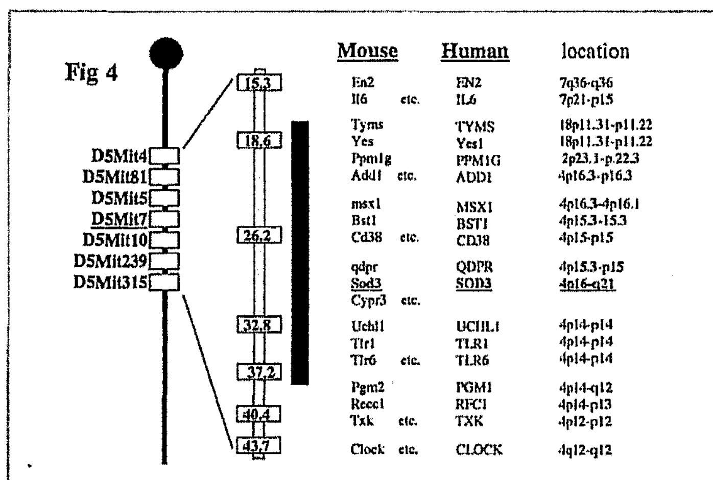
Fig. 4. Composite genetic map of the congenic region for Lys 3. The congenic region on mouse chromosome 5 with the human homologues and their approximate chromosomal locations is shown. The highly probable region (a false positive rate 5% or less) is displayed according to Map Manager QTX 13 software.
