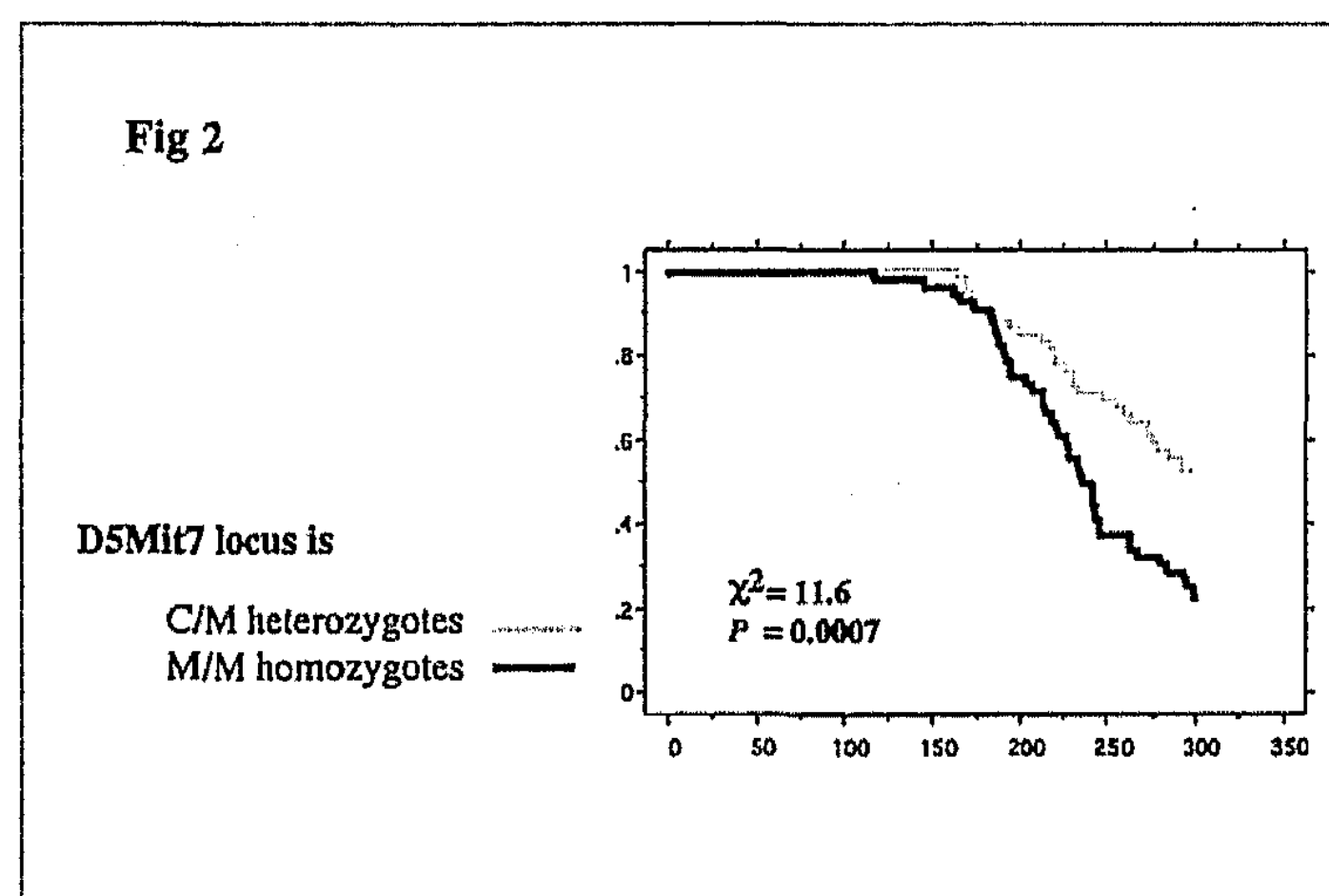
Fig. 2. The cumulative frequencies of thymic lymphoma in congenic mice.
