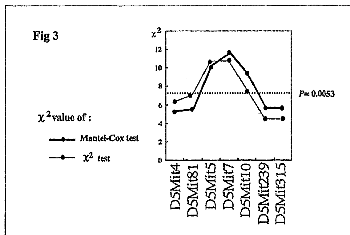
Fig. 3. Location of the resistance locus on chromosome 5. \chi^2 values were obtained by Mantel-Cox test and \chi^2 test with StatView-J 5.0 software. Dotted line shows p=0.0053 ( \chi^2 = 7.767 ) corrected threshold.
