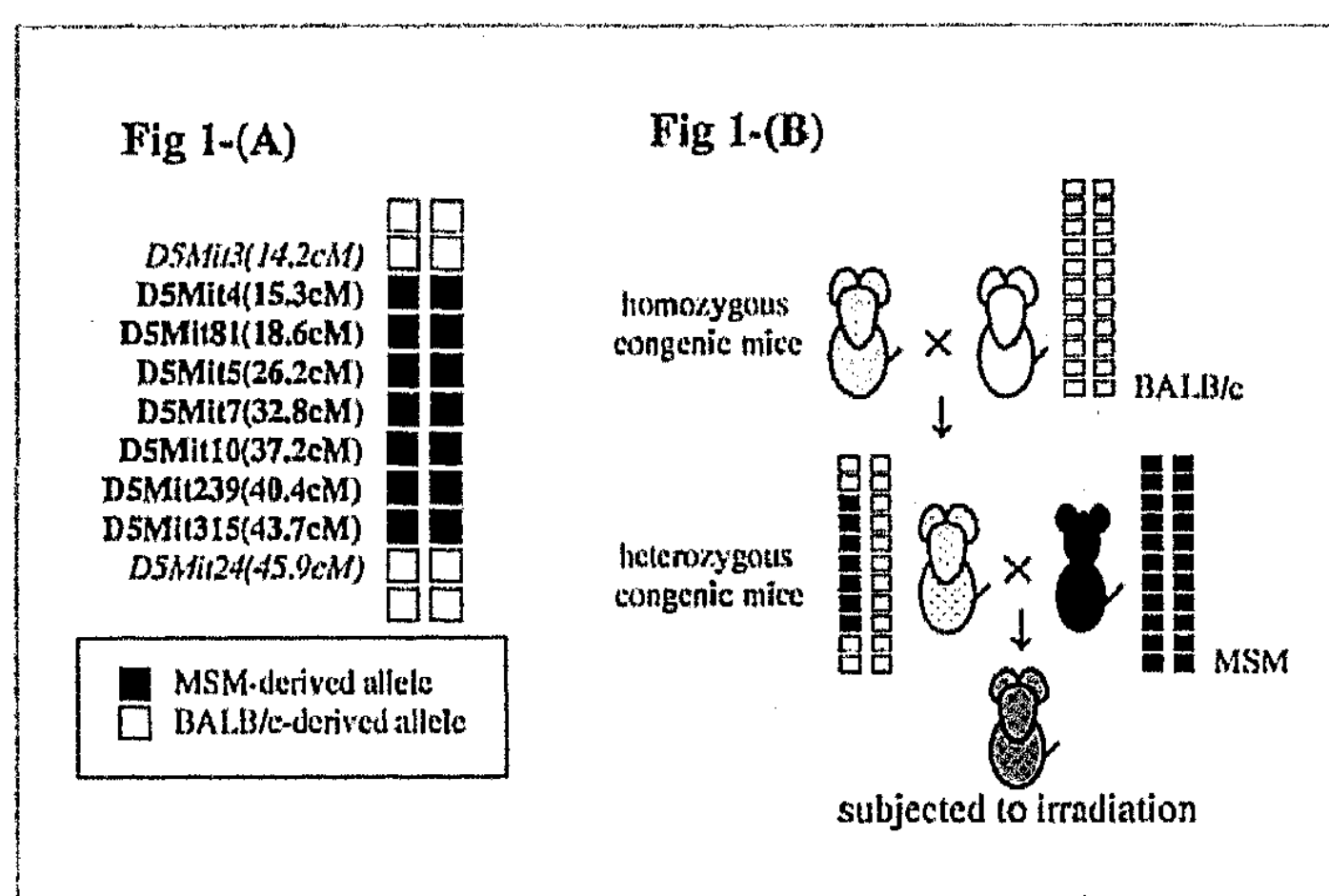
Fig. 1. Schematic draw of a part of chromosome 5 in homozygous congenic mice.
