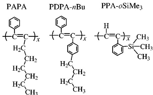
FIG. 1. The molecular structures of PAPA, PDPA- n Bu, and PPA- o SiMe 3 .
