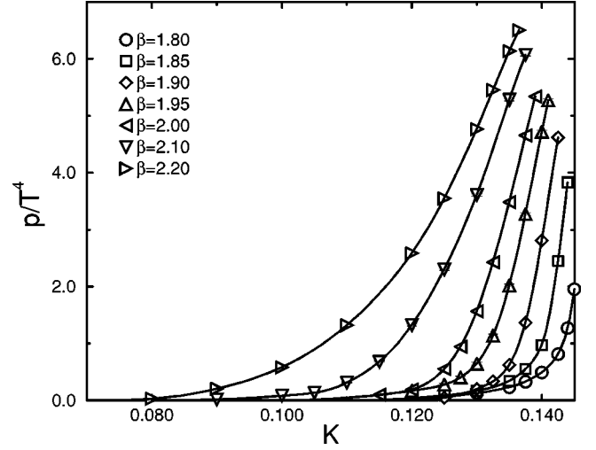
FIG. 12. Pressure as a function of K on a 16^3 \times 4 lattice.
