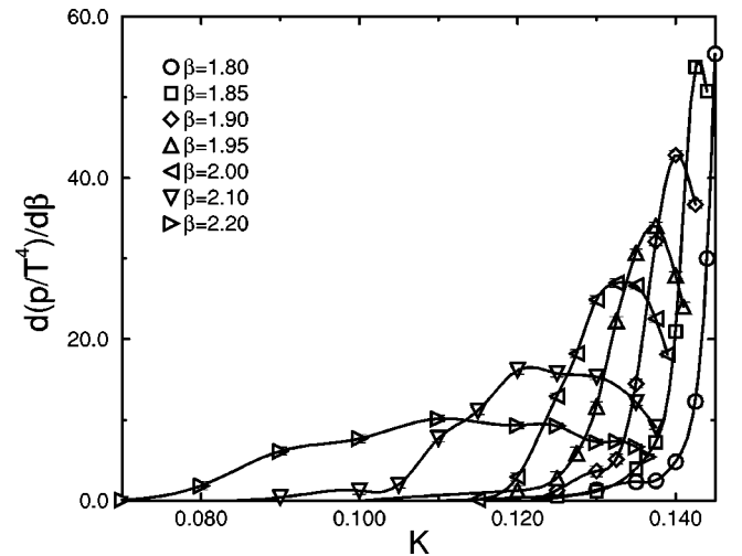
FIG. 13. Derivative of the pressure with respect to \beta as a function of K on a 16^3 \times 4 lattice.
