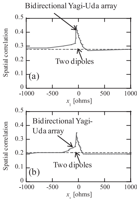
Fig. 8 Median spatial correlation versus the reactance value, x_1 : (a) LOS environment, (b) NLOS environment.
