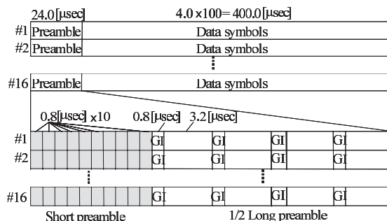
Fig. 2 Frame format of MU-MIMO testbed.
