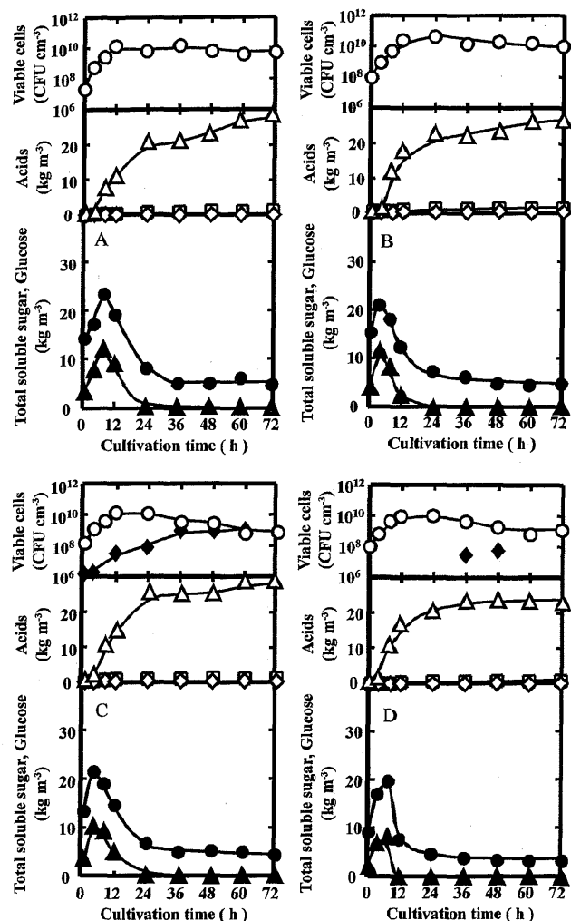
Fig. 2. Production of lactic acid from unsterilized defatted rice bran by SSF using MRS medium (pH 4.5) with (A) strain No. 13, (B) strain No. 16, (C) strain No. 18 and (D) strain No. 19. (○) Viable cells of each lactic acid bacterium inoculated, (◆) viable cells of indigenous lactic acid bacterium, (△) lactic acid, (□) acetic acid, (◇) formic acid, (●) total soluble sugar, (▲) glucose.
